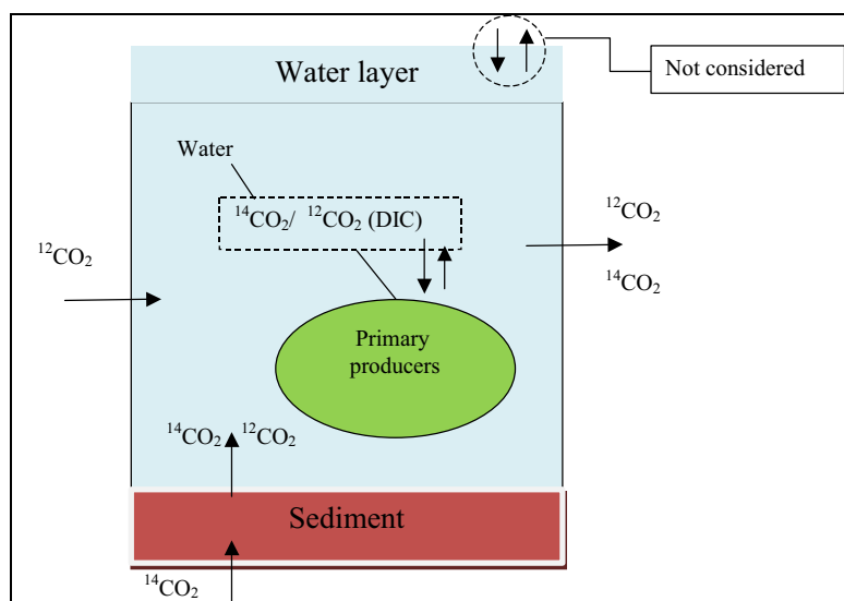
Figure 4.1. Schematic representation of the conceptual model proposed for assessment of exposures to ^{14}\text{C} released from the geosphere to aquatic ecosystems (lakes and sea basins). The arrows represent fluxes of ^{14}\text{CO}_2 and ^{12}\text{CO}_2 . Fluxes between the water layer and the atmosphere are conservatively neglected. The model assumes that the same ^{14}\text{CO}_2 / ^{12}\text{CO}_2 ratio in the water and the primary producers established.
