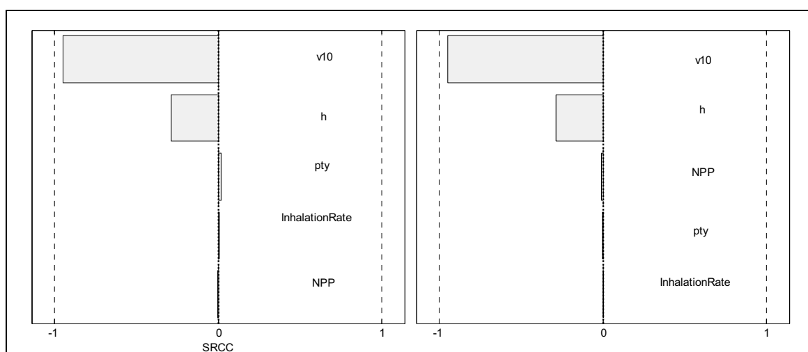
Figure 3.2. Spearman Rank Correlation Coefficients (SRCC) of the total ^{14}\text{C} annual doses per unit release rate obtained for the cases of releases to a forest (left figure) and an agricultural land (right figure). The parameter names are presented in Table 3.1.
