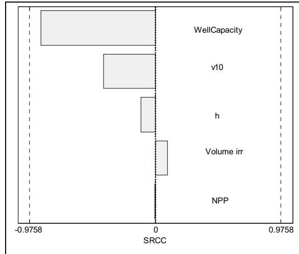
Figure 3.3. Spearman Rank Correlation Coefficients (SRCC) of the ^{14}\text{C}/^{12}\text{C} ratios (specific activities) obtained for the case of irrigation. The parameter names are presented in Table 3.1.
