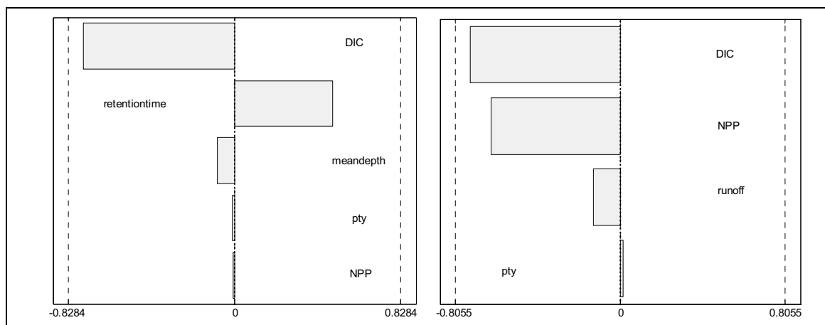
Figure 4.2. Spearman Rank Correlation Coefficients (SRCC) of the total ^{14}\text{C} annual doses per unit release rate obtained for the cases of releases to a sea basin (left figure) and a lake (right figure). The parameter names are presented in Table 4.1.
