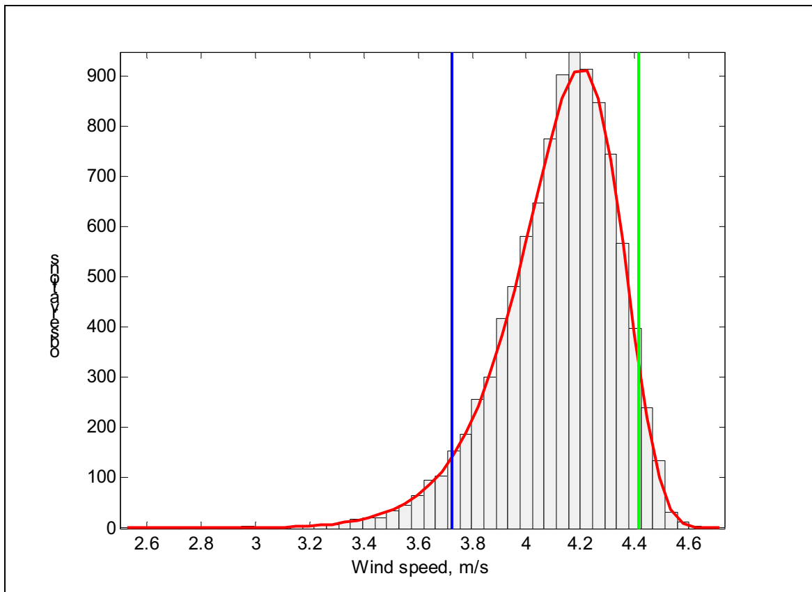
Figure 3.4. Histogram of values of the wind speed at the height of 20 m measured in the Olkiluoto, Finland, and curve obtained from fitting the measured values to a Weibull distribution. The vertical lines indicate the 5 and 95 percentiles of the fitted distribution.
