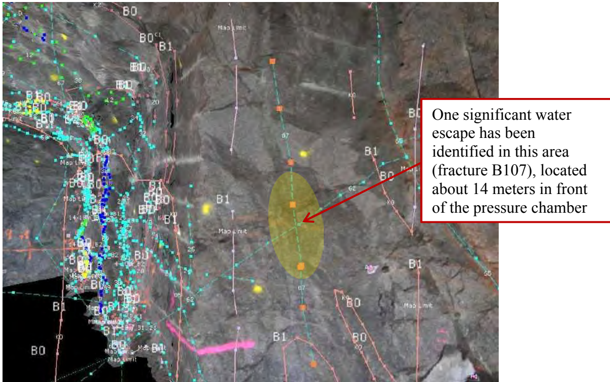
Figure 9-52. Area where leakage was detected in the rock for a water pressure of 3 MPa.
