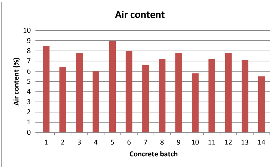
Figure 5-18. Air content, determined at arrival without adjustments, for all batches.
