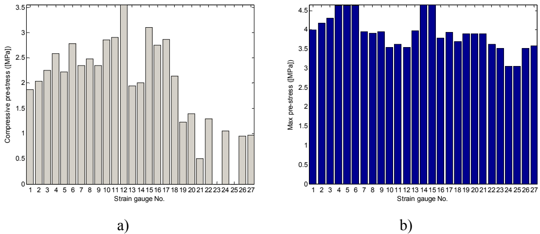
Figure 9-32. Calculated pre-stress in the concrete dome due to cooling and contact grouting. a) Obtained pre-stress based on the strain gauges, b) Max pre-stress based on the temperature variation. From Malm (2014).
