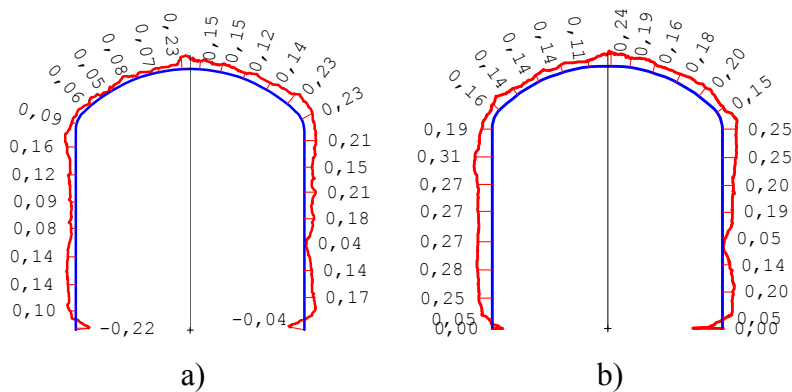
Figure 6-6. Tunnel cross-section at the backfill, a) section 0/016.10 downstream face (i.e. near the filter), b) section 0/016.90 upstream section of backfill (i.e. near the concrete back-wall)
