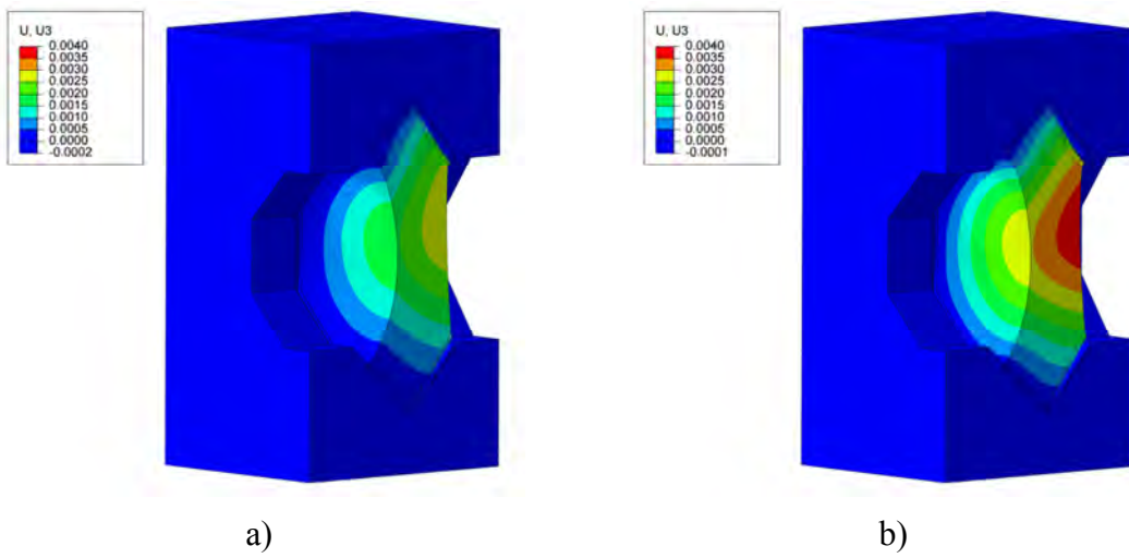
Figure 8-29. Contour of displacement component in the tunnel direction for the full bond model with release of bond during the second cooling cycle, a) prior to the pressure load and b) at 4 MPa water pressure.
