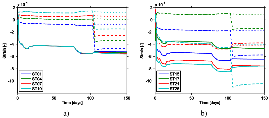
Figure 8-22. Strain output from simulations at sensors locations during the early age of the concrete. Solid lines shows the case of no bond while dashed and dotted lines show the two cases of full bond for the concrete rock interface.
