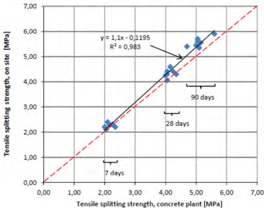
Figure 5-2. Comparison of tensile splitting strength obtained at the concrete plant and at the Äspö Hard Rock Laboratory. From Mathern and Magnusson (2015).
