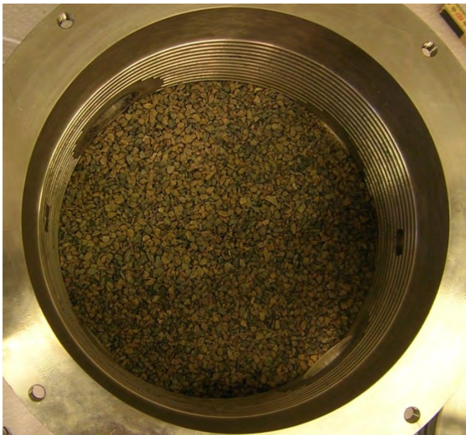
Figure 4-13. The 30 mm layer of 2-4 mm gravel from AB Sydsten employed in the test equipment.
