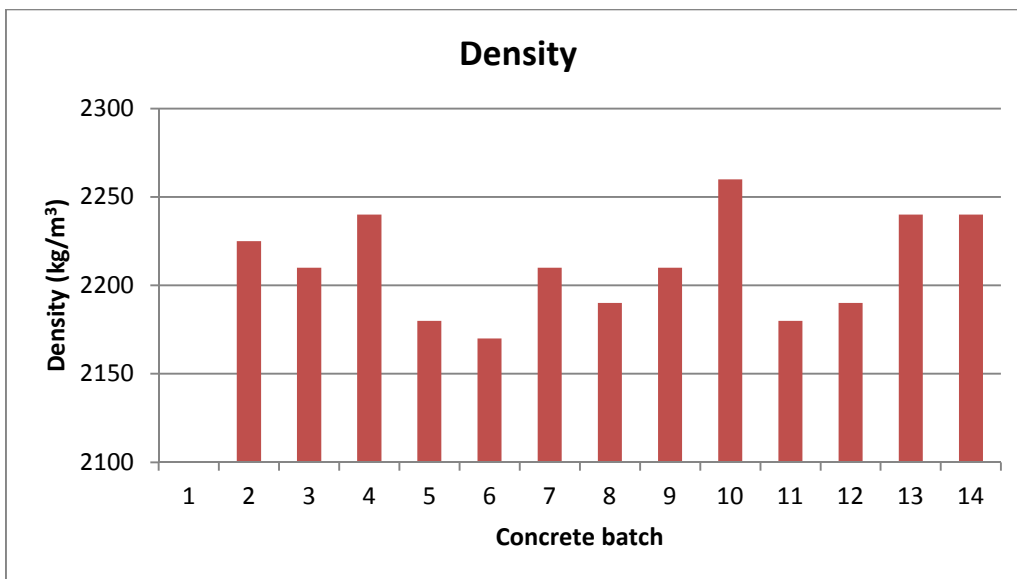
Figure 5-19. Concrete density, determined at arrival without adjustments, for all batches.
