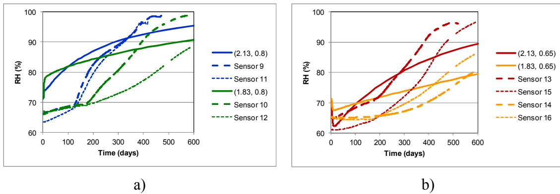
Figure 9-8. Comparison between numerical and measured relative humidity (RH) for the backfill.
