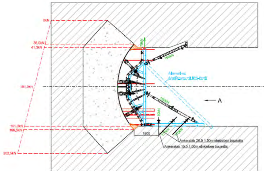
Figure 6-26. Formwork and calculated hydrostatic pressure from poured concrete.
