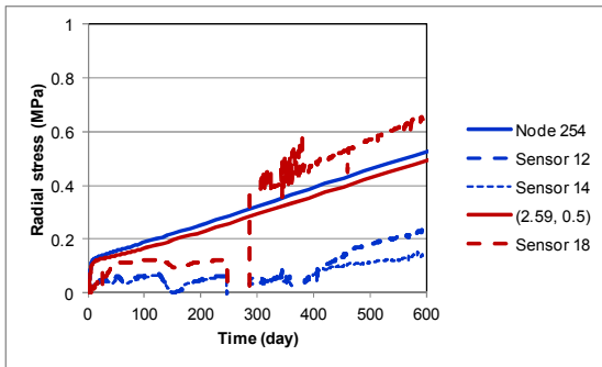
Figure 9-18. Comparison between numerical and measured radial stress in the backfill.
