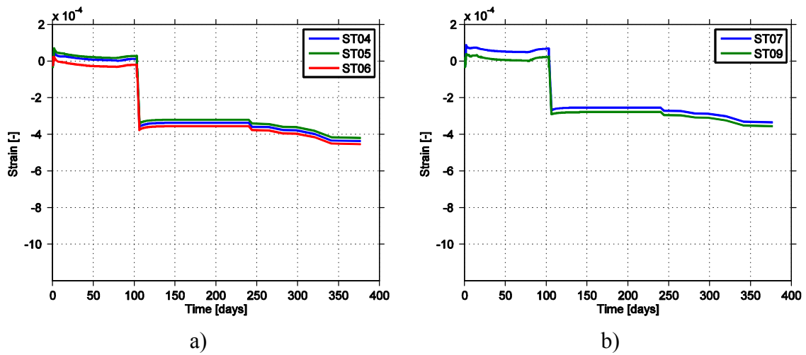
Figure A4-8. Strain output from simulations of the full bond 1 model at sensors in section 2 and 3 including the pressure step.
