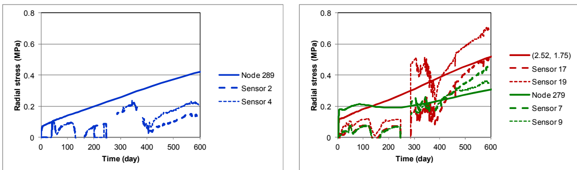
Figure 9-17. Comparison between numerical and measured radial stress in the bentonite seal.
