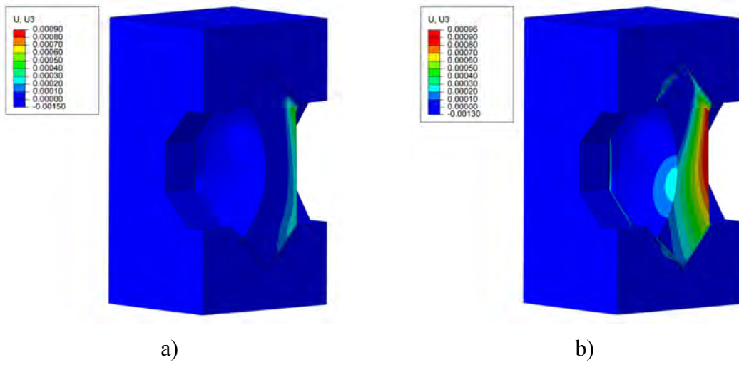
Figure 8-28. Contour of displacement component in the tunnel direction for the no bond model, a) prior to the pressure load and b) at 4 MPa water pressure.
