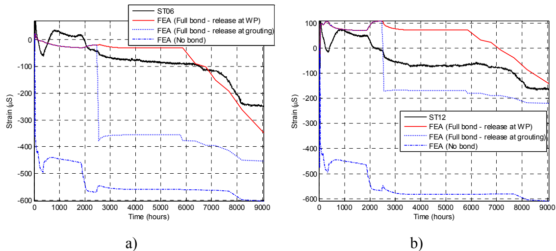
Figure 9-37. Comparison of strain from measurements and numerical analyses for a) ST06 and b) ST12.
