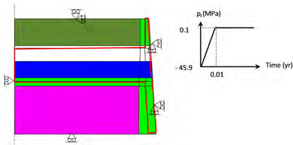
Figure 8-4. Hydraulic surface boundary (red line) defined for the base case model, from Börgesson et al. (2015a).
