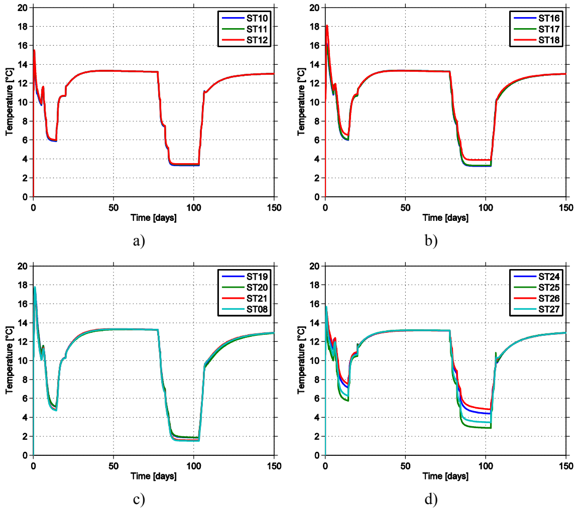
Figure A4-3. Temperature output from simulations at sensors in section 4 and other sensors.
