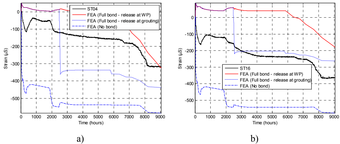
Figure 9-34. Comparison of strain from measurements and numerical analyses for a) ST04 and b) ST16. These represent typical behaviour of the horizontal strain gauges.
