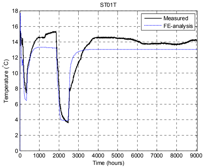
Figure 9-25. Numerical and measured variation in temperature at the location of ST01T.
