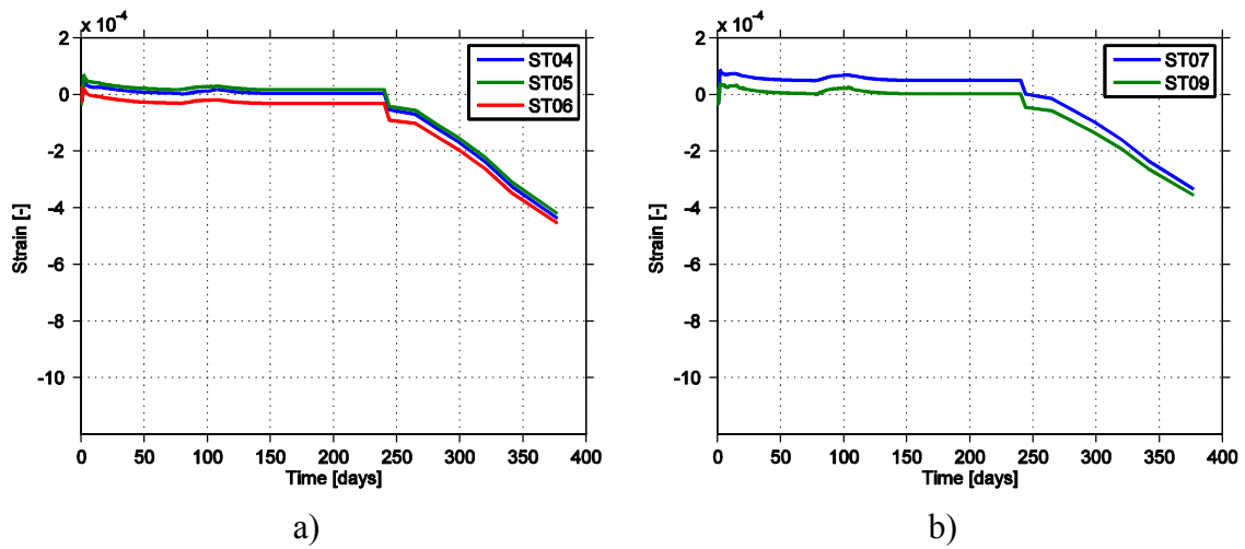
Figure A4-11. Strain output from simulations of the full bond 2 model at sensors in section 2 and 3 including the pressure step.
