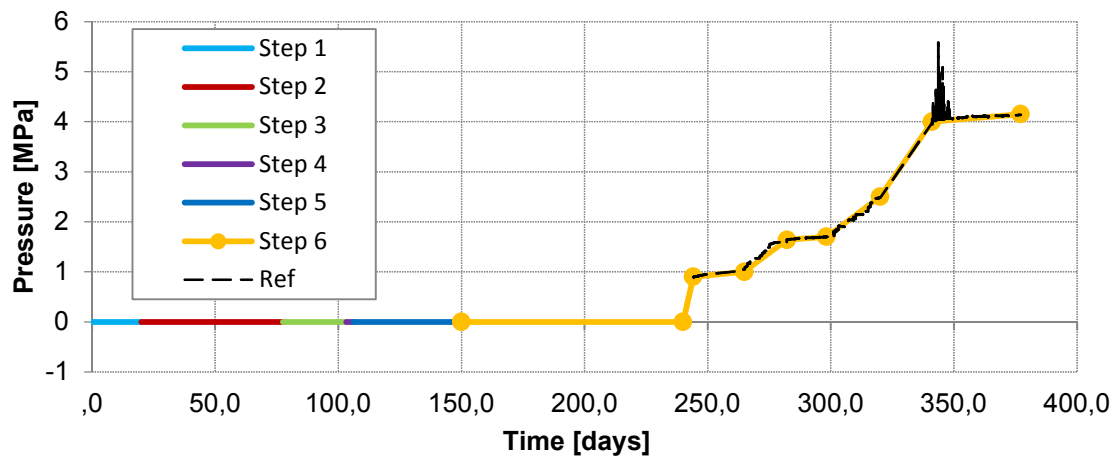
Figure 8-18. Pressure sequence used in the simulations and comparison with measured values in the bentonite seal.
