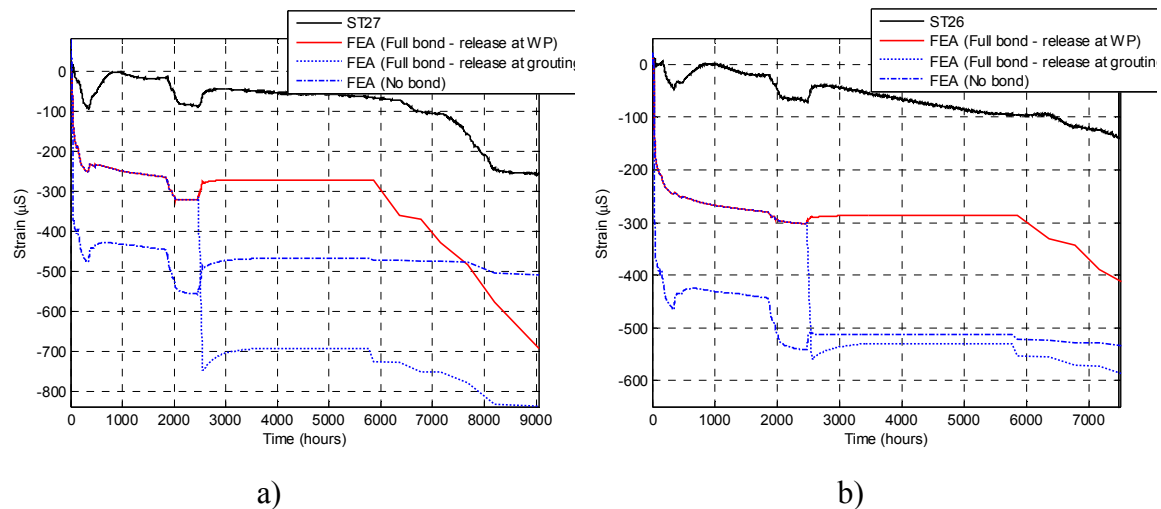
Figure 9-36. Comparison of strain from measurements and numerical analyses for a) ST27 and b) ST26. These represent typical behaviour of the strain gauges close to the slot.
