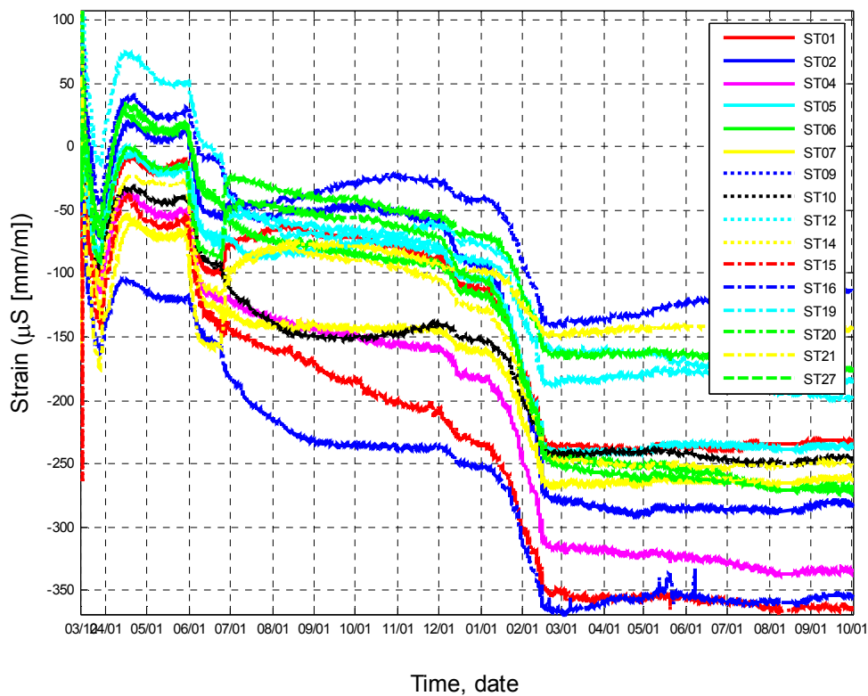
Figure 9-31. Variation in strain for the full measuring period. From Malm (2014).
