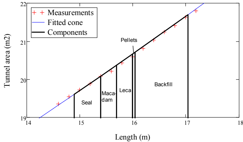
Figure 8-1. Tunnel geometry used in the analytical calculations for the full-scale test, from Börgesson et al. (2015a).
