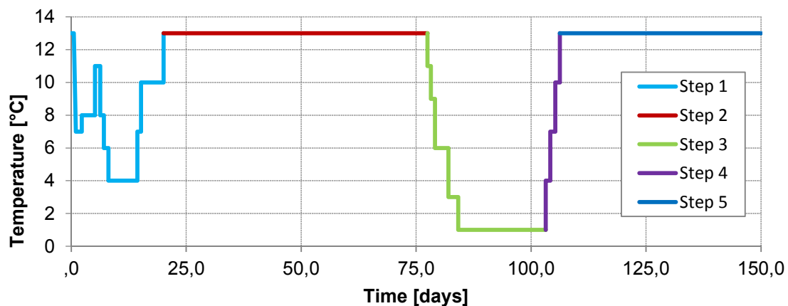
Figure 8-15. Cooling sequence used in the simulations.
