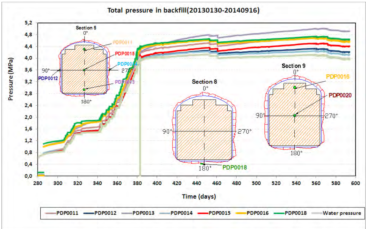
Figure 9-11. Recorded total pressure in the backfill Sections 5, 8 and 9.
