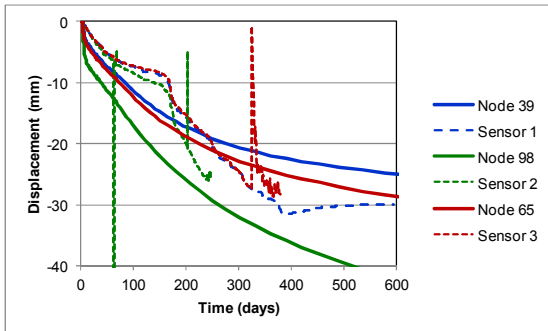
Figure 9-21. Comparison between numerical and measured displacements in the bentonite seal, filter and backfill respectively.
