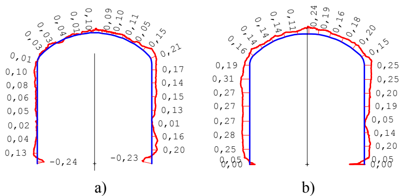
Figure 6-10. Tunnel cross-section at the filter section, a) section 0/015.50 downstream side (i.e. near the bentonite seal), b) section 0/015.90 upstream section of the filter (i.e. near the backfill).
