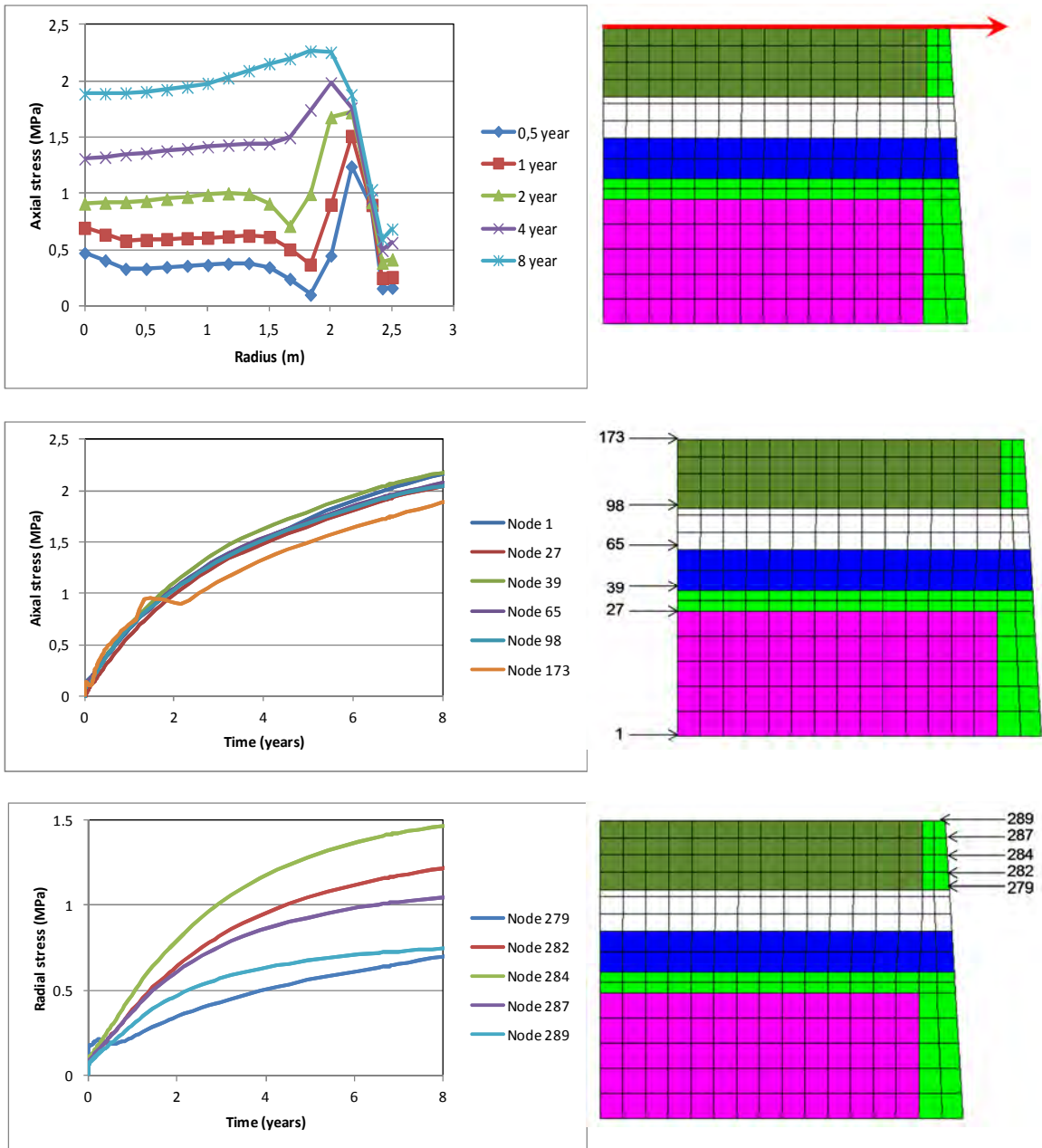
Figure 8-5. Results from the base case analysis showing the axial stress (upper and middle) and the radial stress (lower). From Börjesson et al. (2015a).
