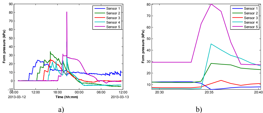
Figure 9-22. Measured form pressures for the five pressure sensors on formwork. a) during the whole time period and b) zoomed in on the pressure spike.
