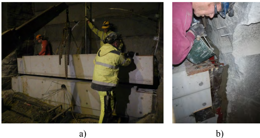
Figure 6-17. Installation of a concrete beam, a) lifting it into place, b) filling of gap between beam end and the rock wall.
