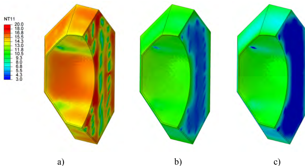
Figure 8-21. Simulated temperature fields in the concrete dome at a) 42 hours, b) 14 days and c) 100 days from casting.
