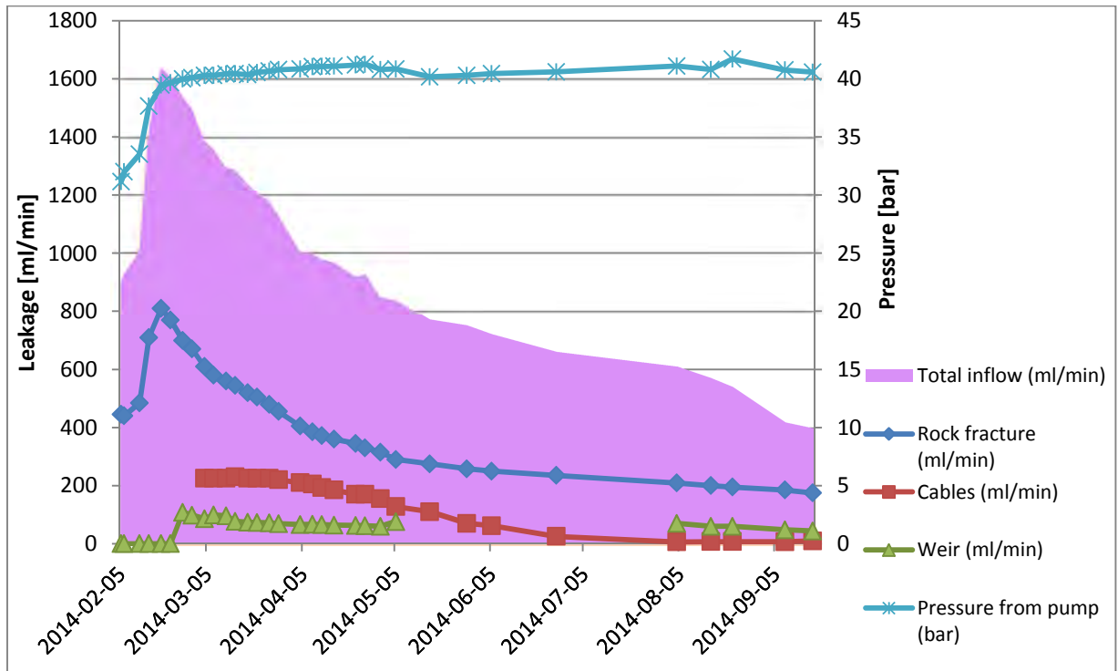
Figure 9-54. Measurements of leakage together with total water injection flow needed to keep the water pressure stable near at 4 MPa (about 40 bar).
