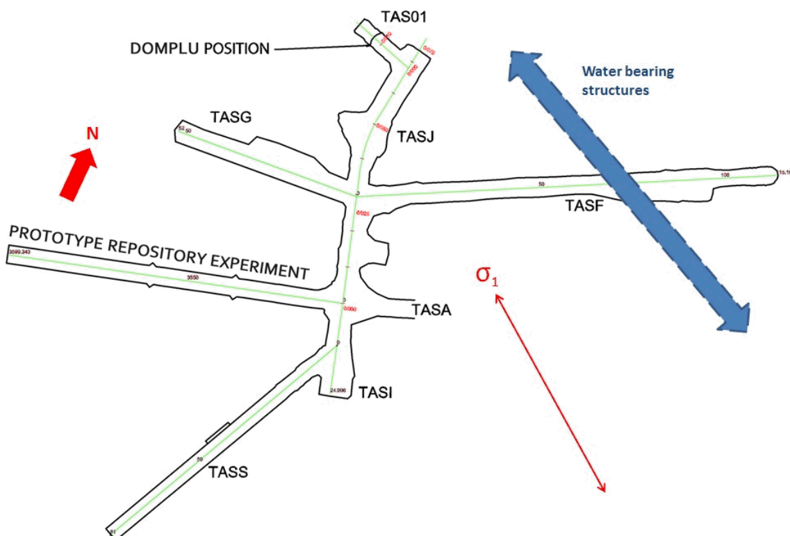
Figure 3-2. Layout of Äspö HRL at level - 450 m and the location of the DOMPLU full-scale plug test site TAS01. The major principal stress direction ( \sigma_1 ) and the main direction for the water bearing structures have been marked in the figure.
