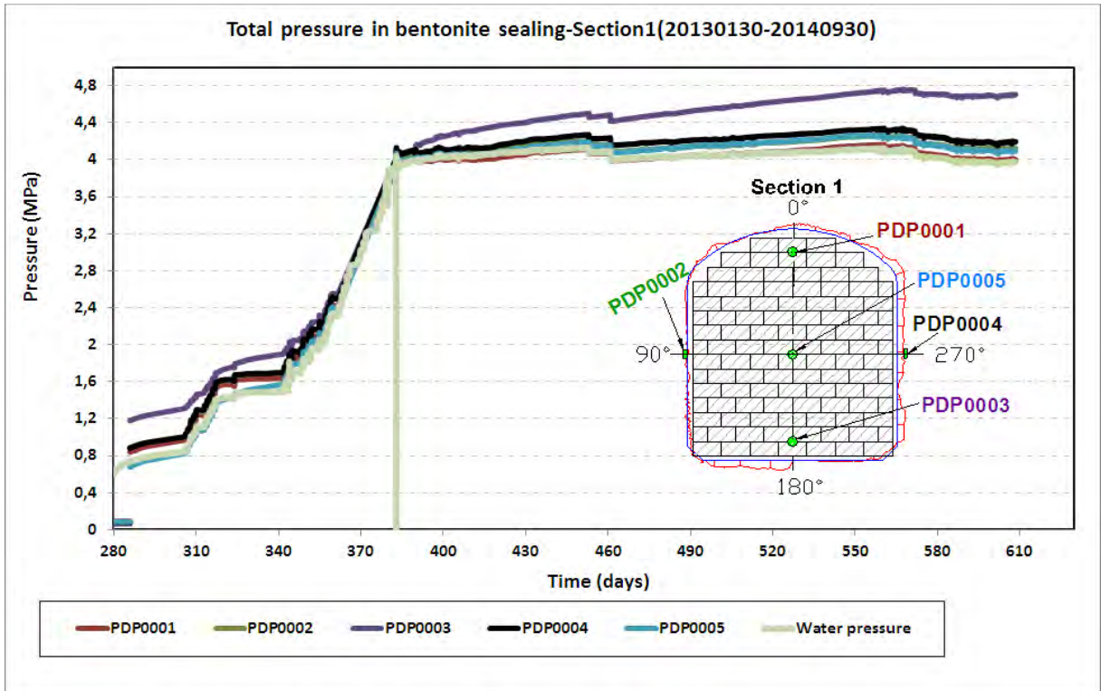
Figure 9-9. Total pressure in Section 1 in the bentonite seal.
