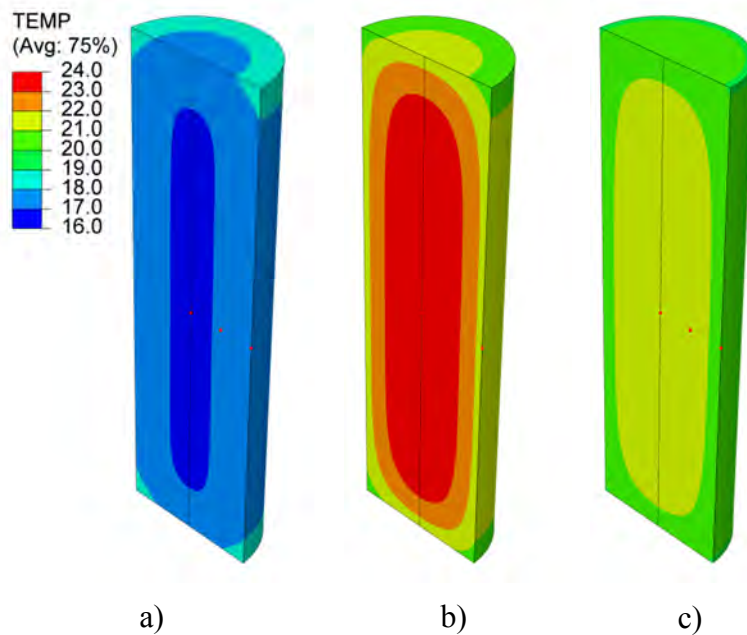
Figure 8-9. Modelled temperature distribution in the concrete cylinder after a) 6 h, b) 40 h and c) 100 h.
