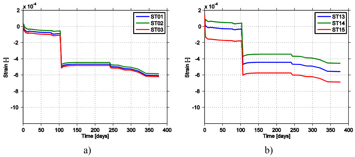
Figure A4-7. Strain output from simulations of the full bond 1 model at sensors in section 1 including the pressure step.
