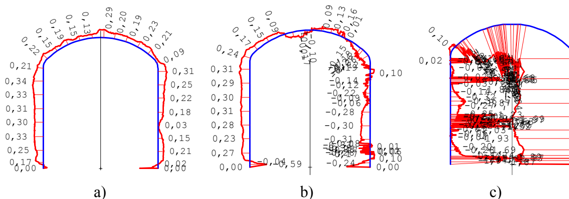
Figure 6-3. Tunnel cross-section at the concrete wall, a) section 0/017.10 downstream front face of the back-wall, b) section 0/017.50 last horse-shoe shaped section of TAS01, c) section 0/017.90 the tunnel face of TAS01. Figures 6-3b and 6-3c are cluttered by numbers due to measuring contact with the intact rock.
