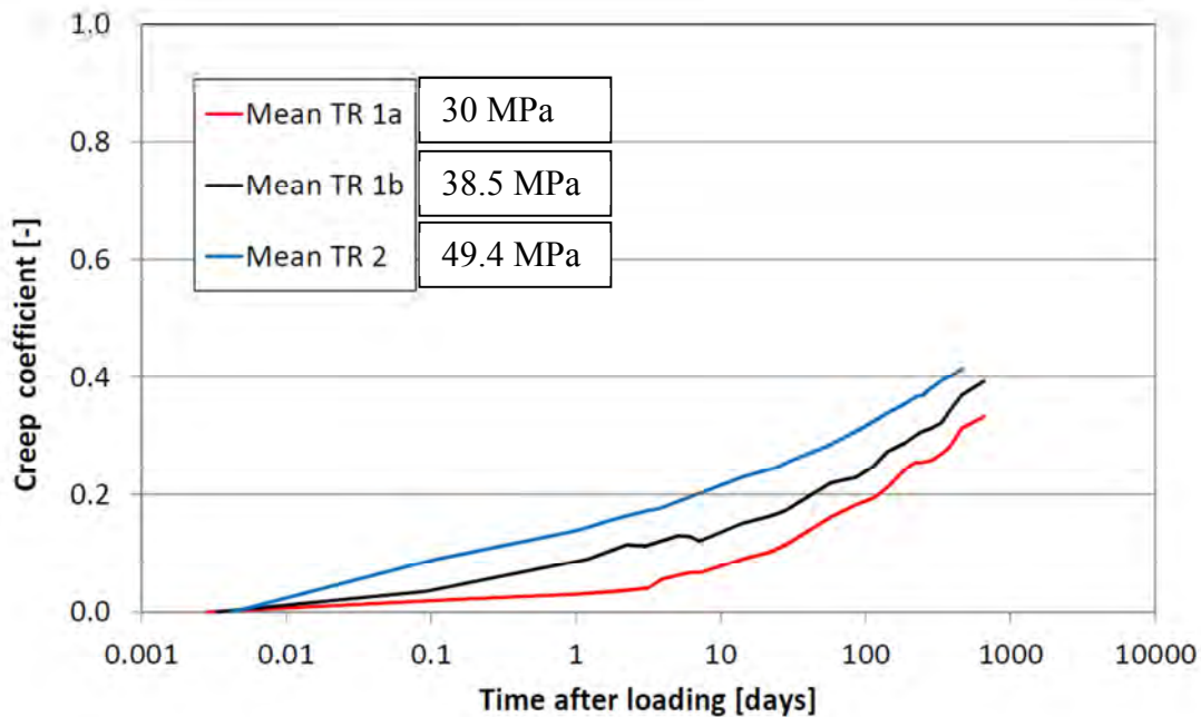
Figure 5-14. Mean value of the creep coefficient with time for TR 1a, TR 1b and TR2. (From Flansbjer and Magnusson 2014a).
