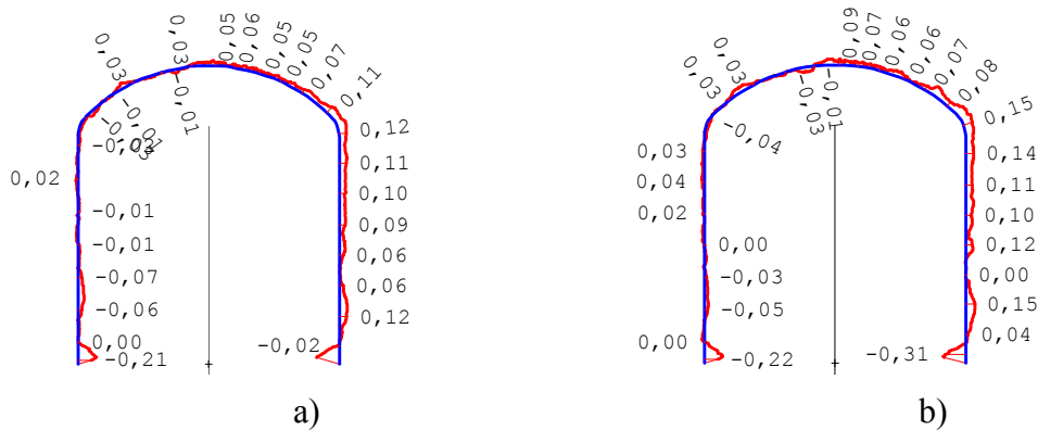
Figure 6-16. Tunnel cross-section at the concrete delimiter position, a) section 0/014.70 downstream section (i.e. near the concrete dome), b) section 0/014.90 corresponds to the upstream delimiter face (adjacent to the bentonite seal).
