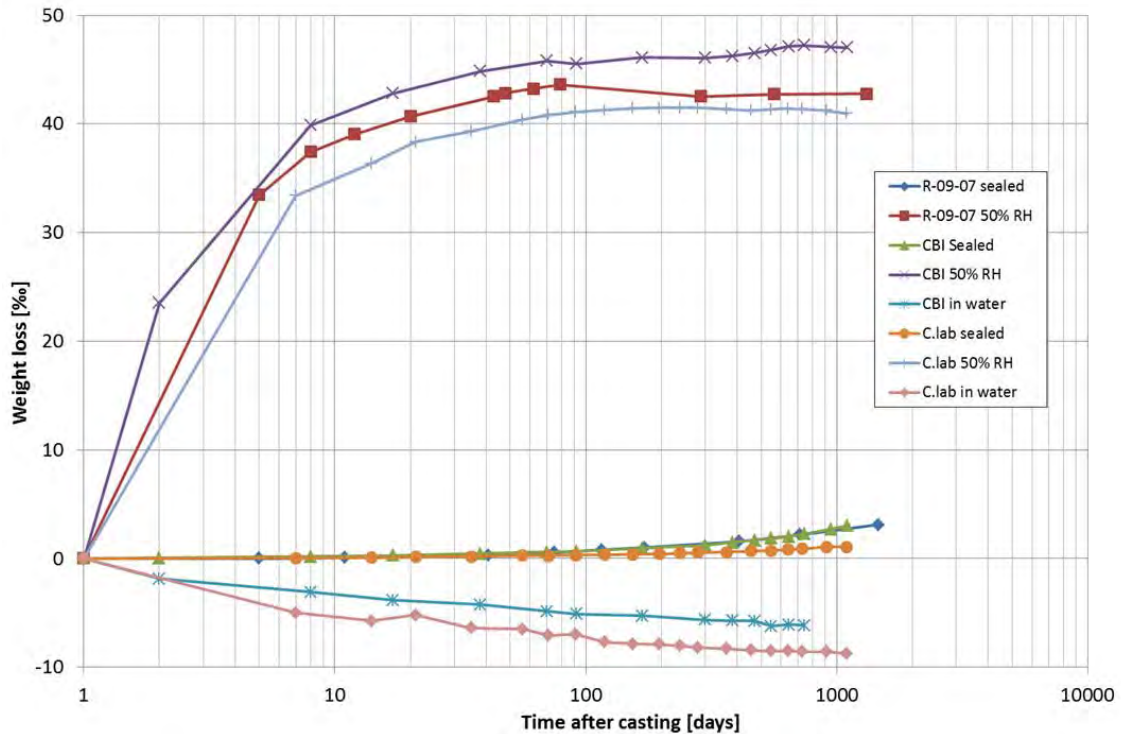
Figure 5-12. Average weight loss of the specimens tested at CBI and C.lab. The older results from the testing at CBI, presented in Vogt et al. (2009), are also shown as comparison. (From Mathern and Magnusson 2015).
