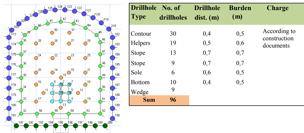
Figure 3-4. Drill and charge plan for DOMPLU test tunnel TAS01.
