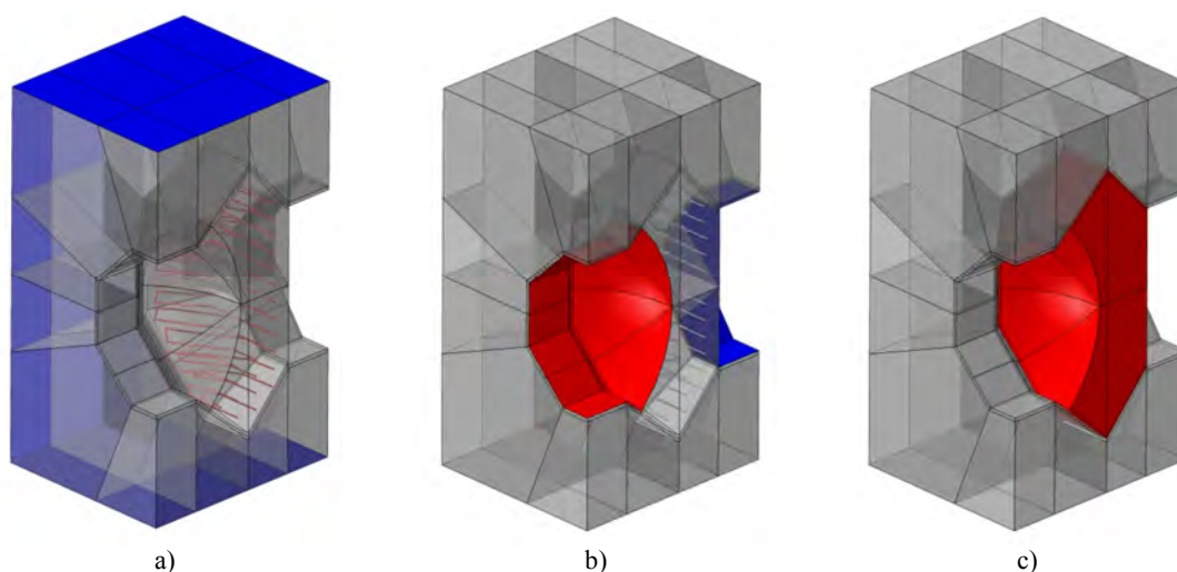
Figure 8-13. Boundary conditions, a) shows regions with prescribed temperature, b) shows regions with convective boundaries and c) show regions which are assigned a temperature load.
