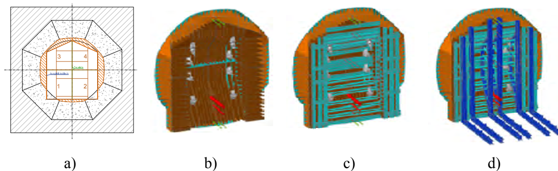
Figure 6-23. Designed formwork used for casting the concrete dome plug.
