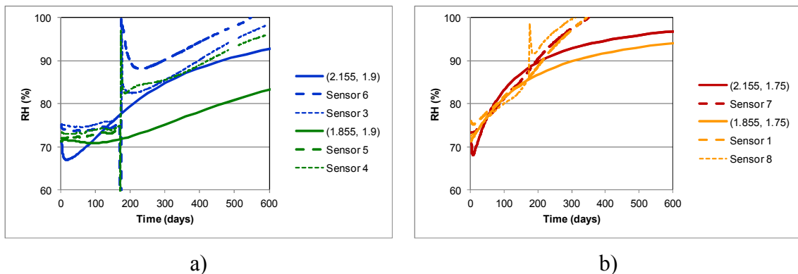
Figure 9-7. Comparison between numerical and measured relative humidity (RH) for the bentonite seal.
