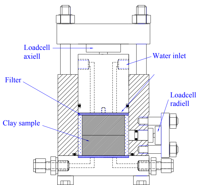
Figure 4-5. Schematic drawing of the test equipment.
