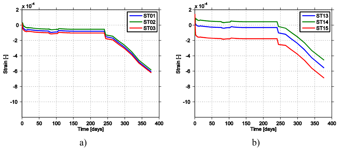
Figure A4-10. Strain output from simulations of the full bond 2 model at sensors in section 1 including the pressure step.
