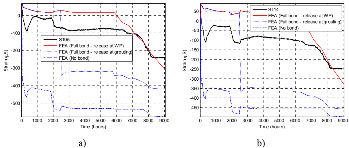
Figure 9-35. Comparison of strain from measurements and numerical analyses for a) ST05 and b) ST14. These represent typical behaviour of the inclined strain gauges.
