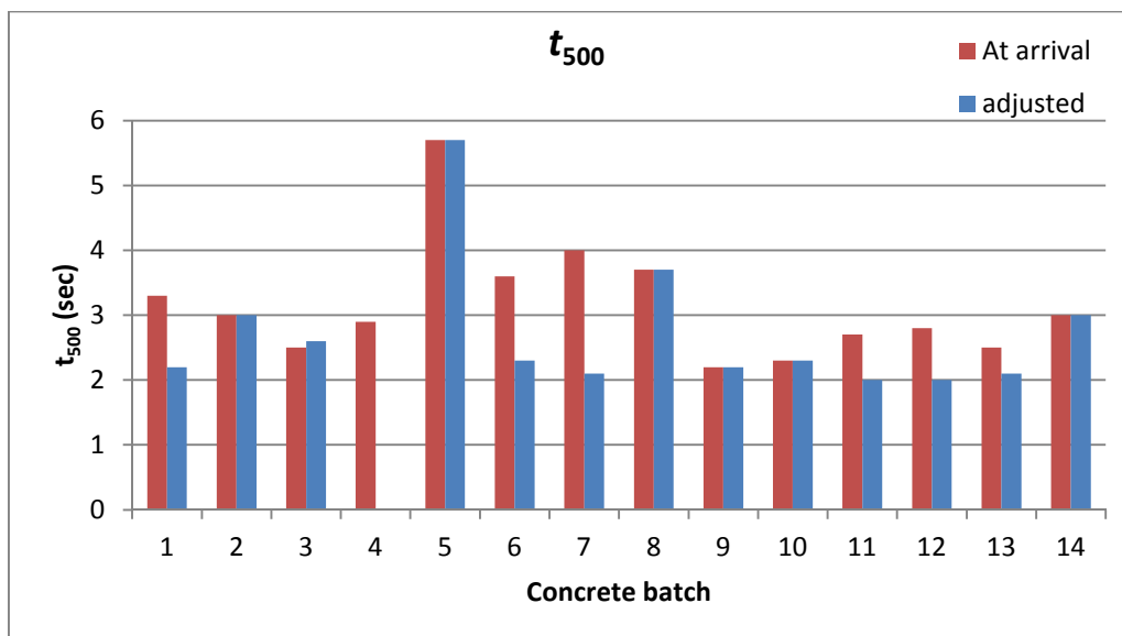
Figure 5-21. t_{500} , determined at arrival without adjustments and after adjustments, for all batches. In case identical values are presented for one batch, e.g. no.2, no adjustments were done.
