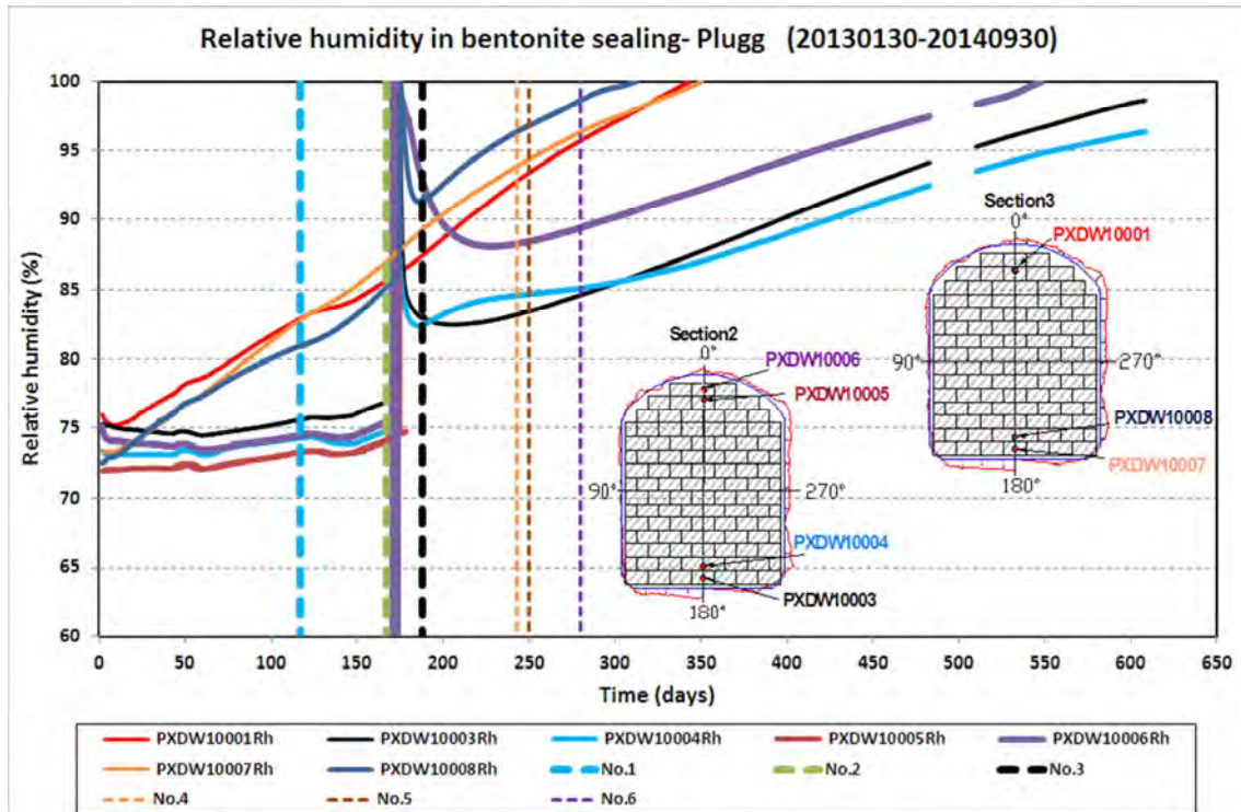
Figure 9-3. Relative humidity recordings in the bentonite seal. Activities associated with testing (see section 9.1.1) are identified as “No.1 through No.6”.
