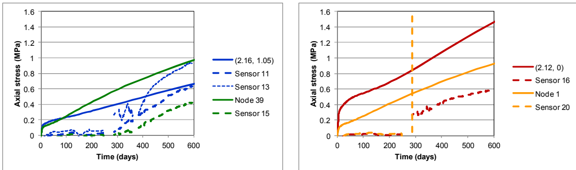
Figure 9-15. Comparison between numerical and measured axial stress in the backfill.
