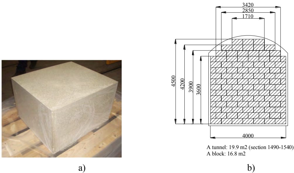
Figure 6-13. a) MX-80 block for the bentonite seal. b) Schematic arrangement of bentonite blocks in the bentonite seal.
