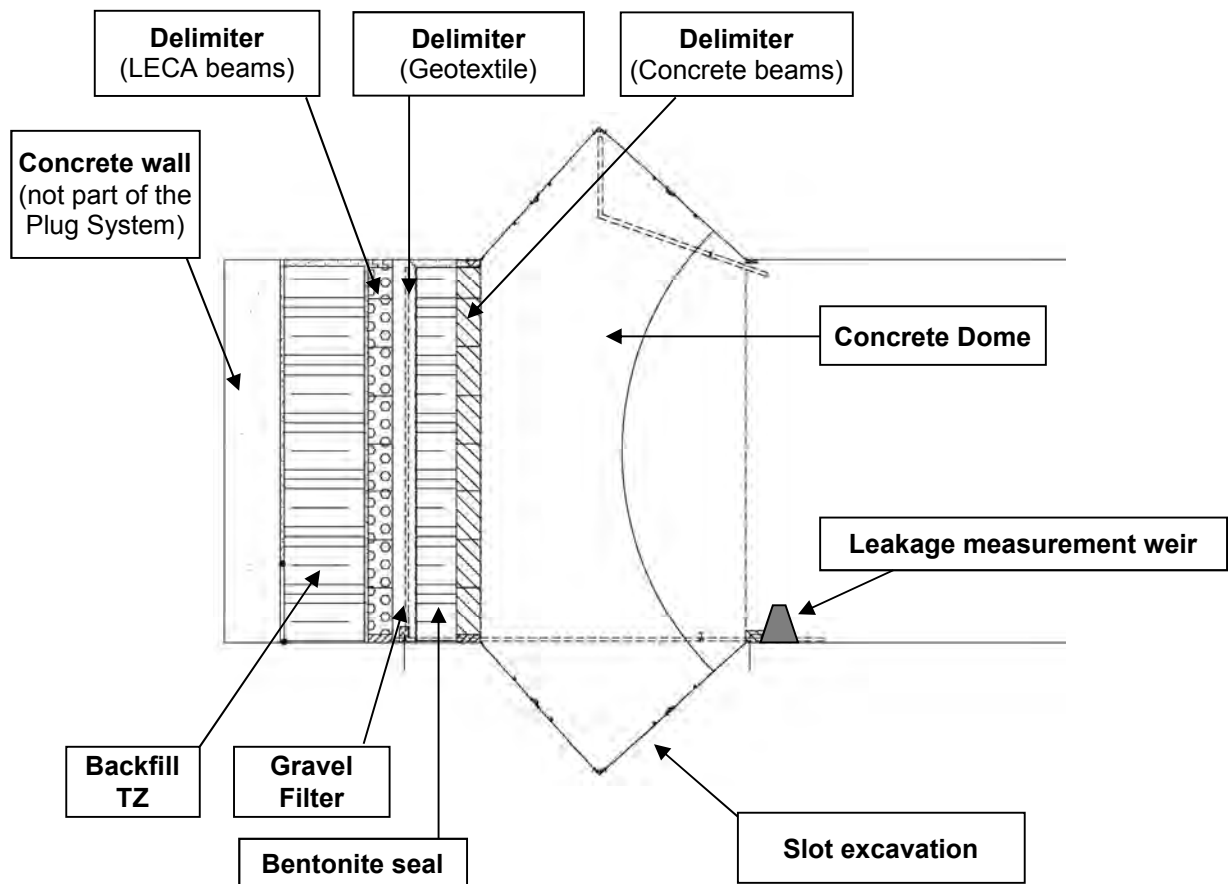
Figure 1-3. Illustration of the structural components that make up the Plug System. Note that the concrete wall is not a plug system component but a structural part of the DOMPLU experiment.
