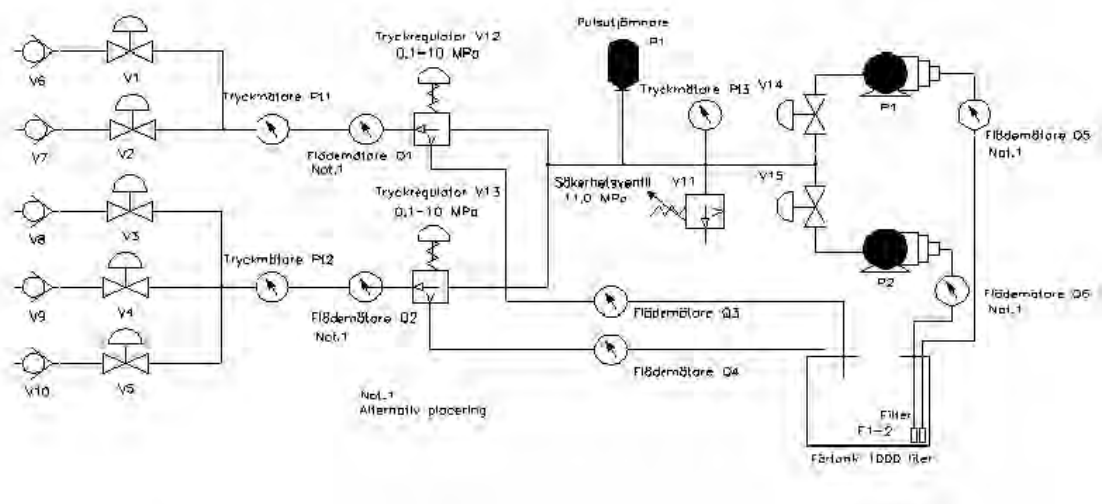
Figure 7-9. Pressurization system flowchart. (Text in Swedish)
