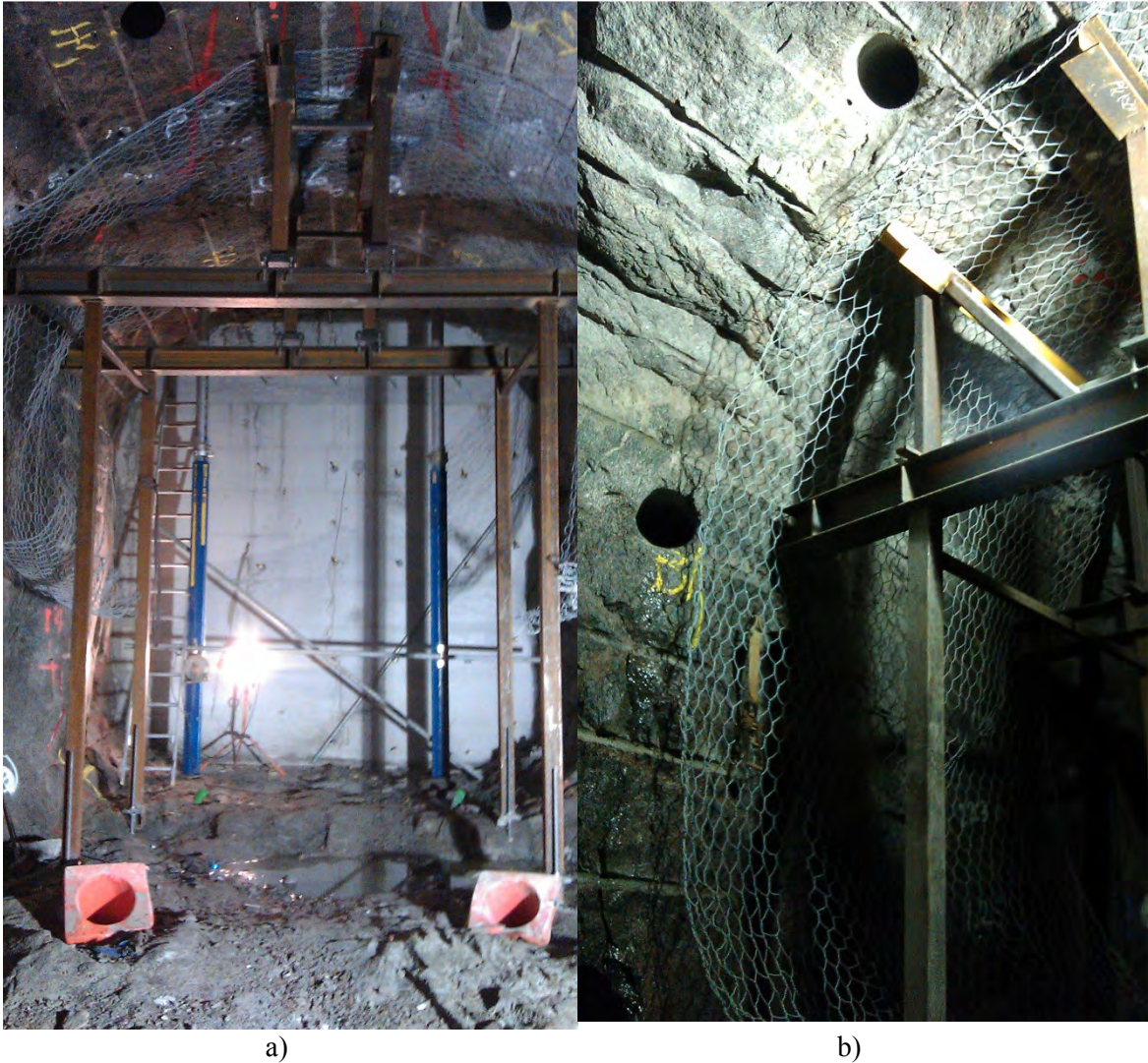
Figure 3-9. a) Photo of the erected safety scaffolding including a tunnel mesh to protect workers from falling rocks b) Detail of the scaffolding with two of the Ø250 mm boreholes visible.
