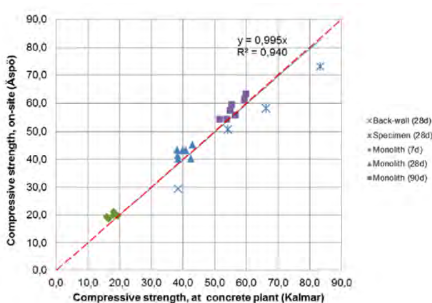
Figure 5-3. Comparison of tested compressive strength on concrete cubes cast at the concrete plant in Kalmar and on site at the Äspö Hard Rock Laboratory. From Mathern and Magnusson (2015).
