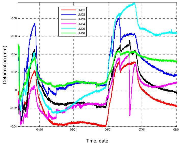
Figure 9-43. Variation in relative displacement between concrete dome and rock. From Malm (2014).
