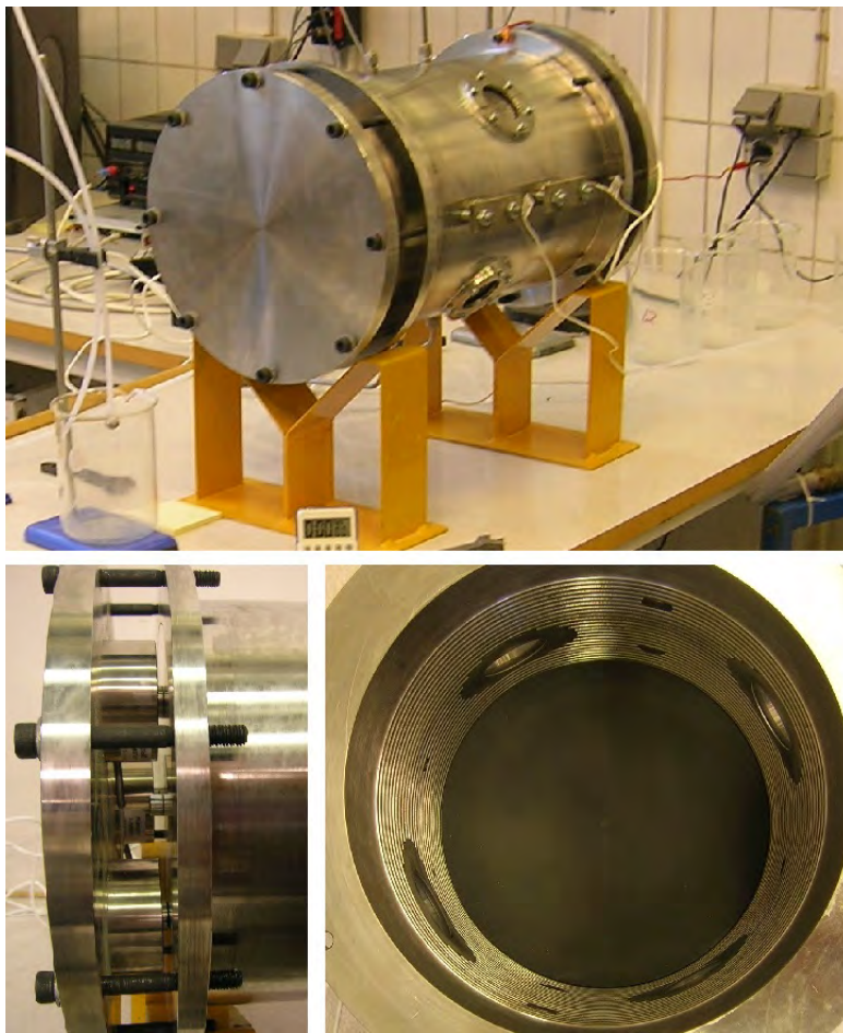
Figure 4-7. The DOMPLU scale model test equipment, from Börgesson et al. (2015a).
