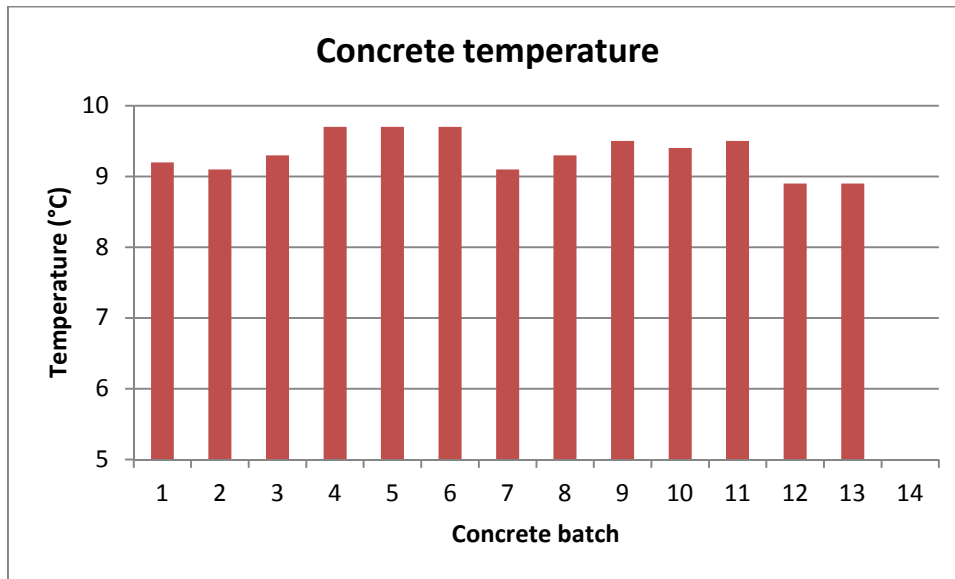
Figure 5-17. Concrete temperature, determined at arrival without adjustments, for all batches
