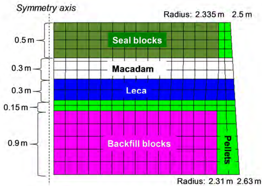
Figure 8-3. Geometry and mesh used for the base case model, after Börgesson et al. (2015a).
