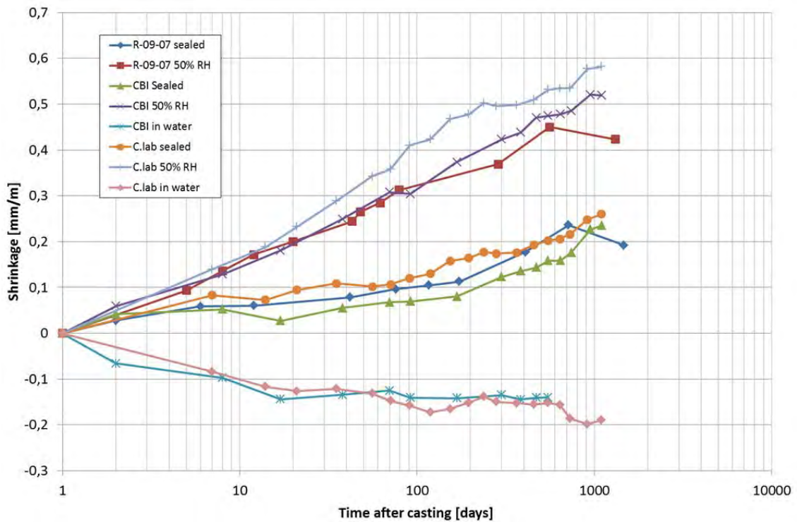
Figure 5-11. Average shrinkage of the specimens tested at CBI and C.lab. The older results from the testing at CBI, presented in Vogt et al. (2009), are also shown as comparison. (From Mathern and Magnusson 2015).
