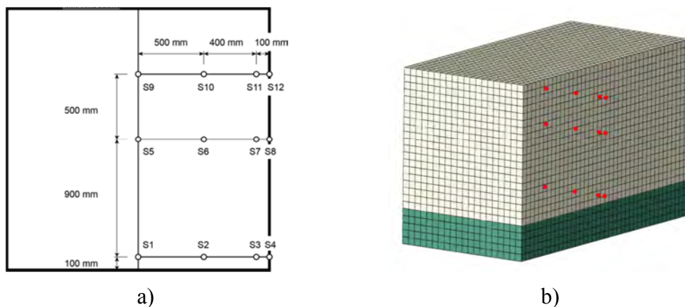
Figure 8-10. Distribution of temperature sensors shown in a) midsection of the test body and b) in the FE-model.
