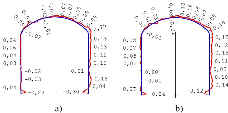
Figure 6-14. Tunnel cross-section at the backfill, (a) section 0/015.10 downstream part of the seal (near the concrete beams), (b) section 0/015.30 upstream part of the seal (near the filter).
