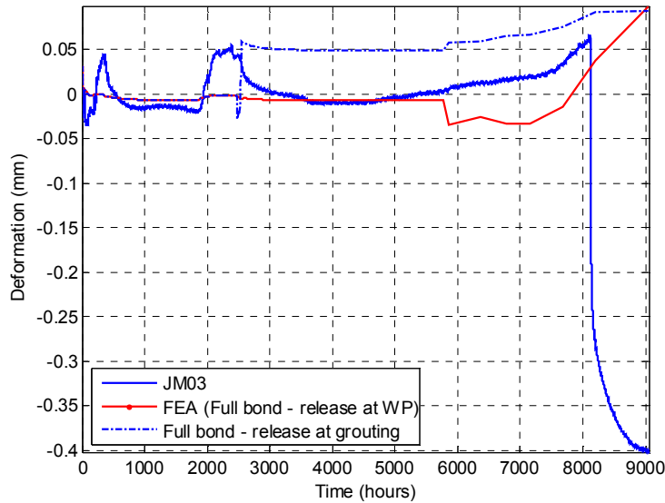
Figure 9-45. Comparison of measured and calculated relative displacement for the joint-meter JM03 (located in the top of the dome).
