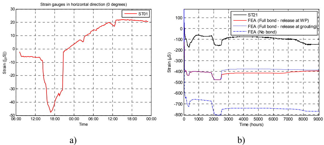
Figure 9-38. Behaviour of Geokon strain gauges. a) early age behaviour of ST01, b) variations in strain of ST21.
