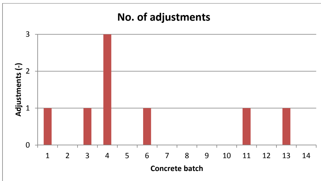
Figure 5-22. Number of required adjustments for all batches.
