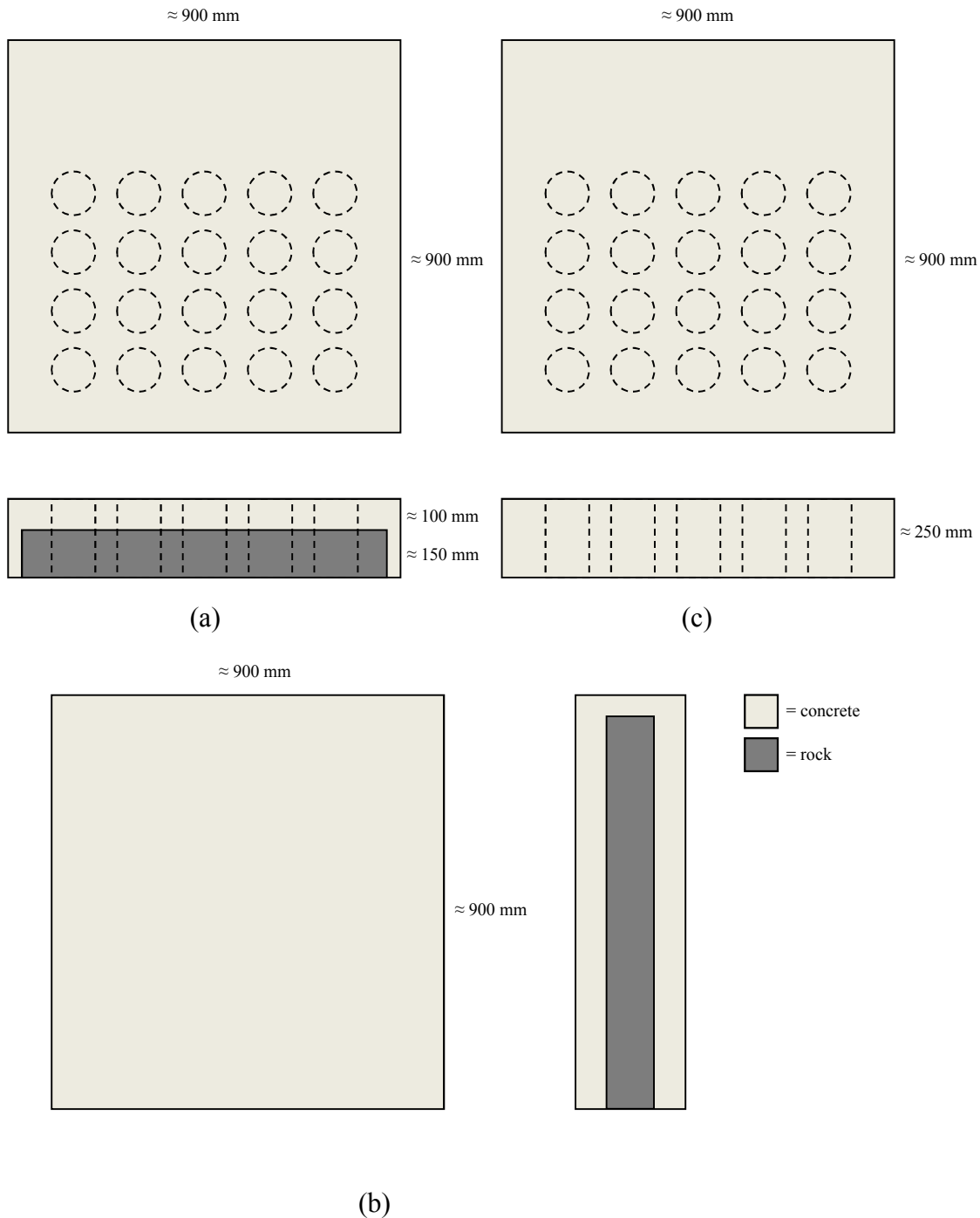
Figure 5-6. Illustration of the prepared a) horizontal rock-concrete blocks, b) vertical rock-concrete blocks and c) plain concrete blocks. (From Flansbjerg and Magnusson 2014b).
