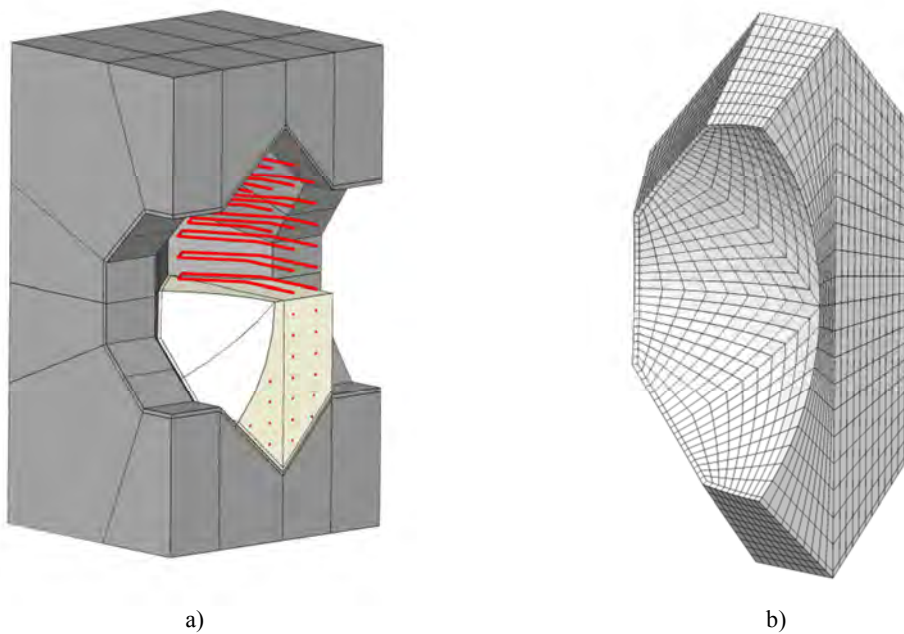
Figure 8-12. a) Geometry and b) mesh of the FE-model.
