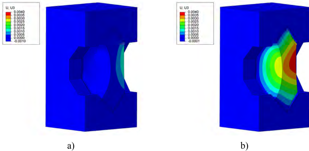
Figure 8-30. Contour of displacement component in the tunnel direction for the full bond model with release of bond at the application of water pressure, a) prior to the pressure load and b) at 4 MPa water pressure.
