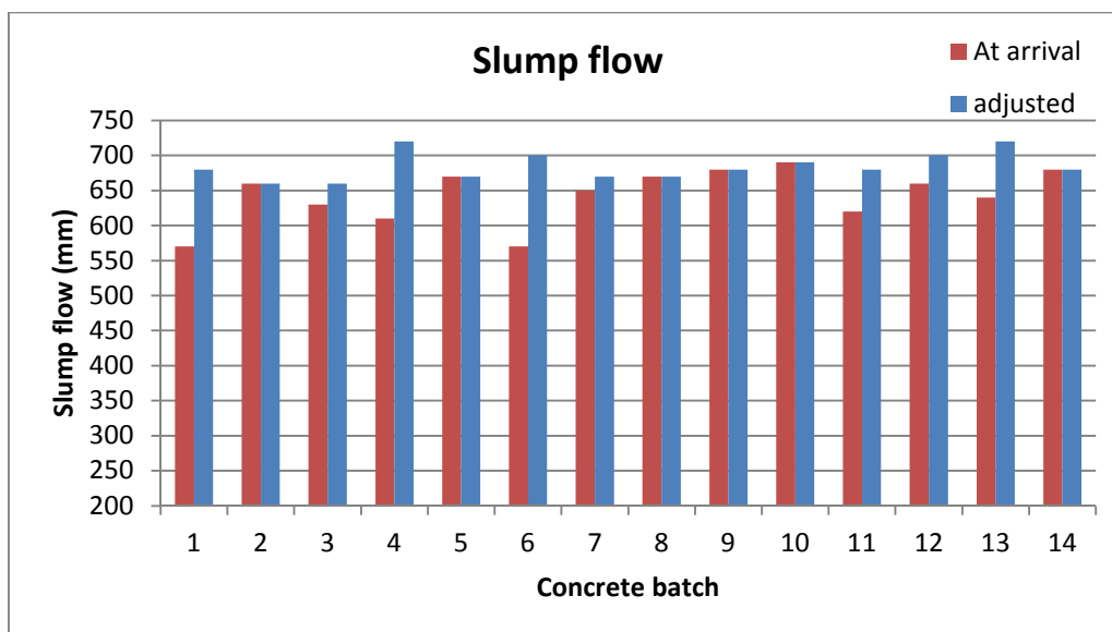
Figure 5-20. Slump flow, determined at arrival without adjustments and after adjustments, for all batches. In case identical values are presented for one batch, e.g. no.2, no adjustments were done.
