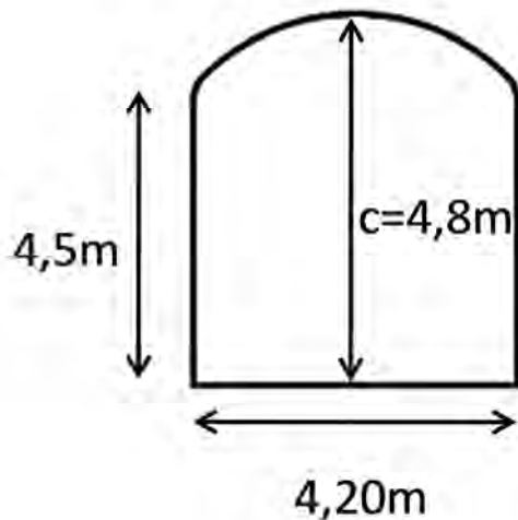
Figure 3-1. Principle tunnel dimensions of a KBS-3V deposition tunnel.
