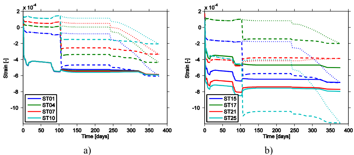
Figure 8-25. Strain output from simulations at sensors locations including pressurisation. Solid lines shows the case of no bond while dashed and dotted lines show the two different cases of full bond for the concrete rock interface.
