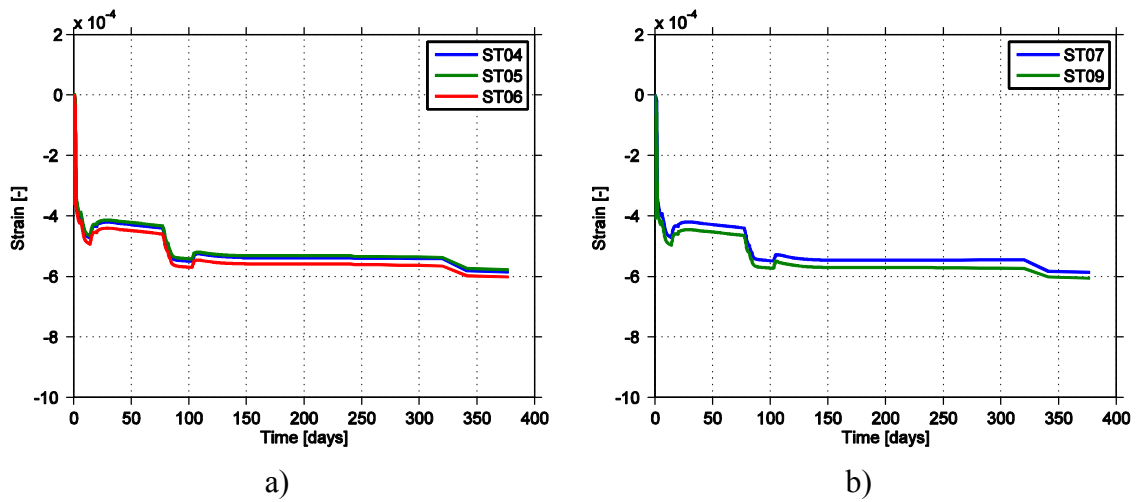
Figure A4-5. Strain output from simulations with no bond at sensors in section 2 and 3 including the pressure step.
