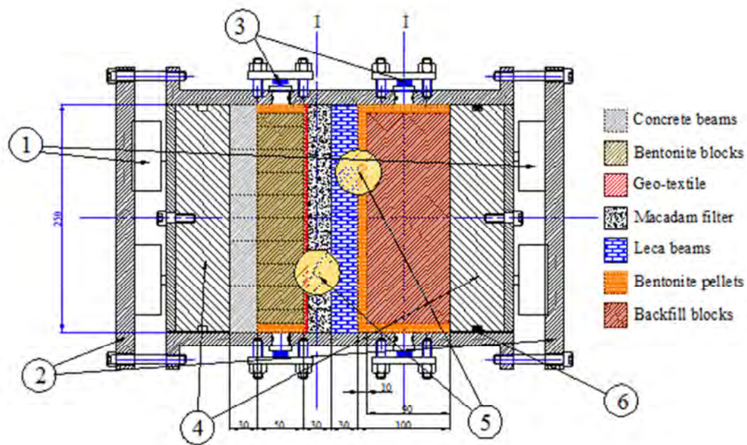
Figure 4-8. Cross section of the scale model used for testing. The different components are explained by the legend above. The axial load cells (1) are held in place by steel plates (2). Radial load cells (3) are placed on the bentonite sealing and the backfill. There is a PVC plate piston (4) on each side of the components. The PVC plate piston to the left is slightly smaller than the tube and represents a non-hardened concrete dome that allows for leakage. The PVC plate piston to the right is sealed with an O-ring (6) to prevent water from leaking in that direction. On each side of the tube there are two windows (5) showing bentonite sealing, geotextile, gravel (macadam), LECA and backfill. From Börgesson et al. (2015a).
