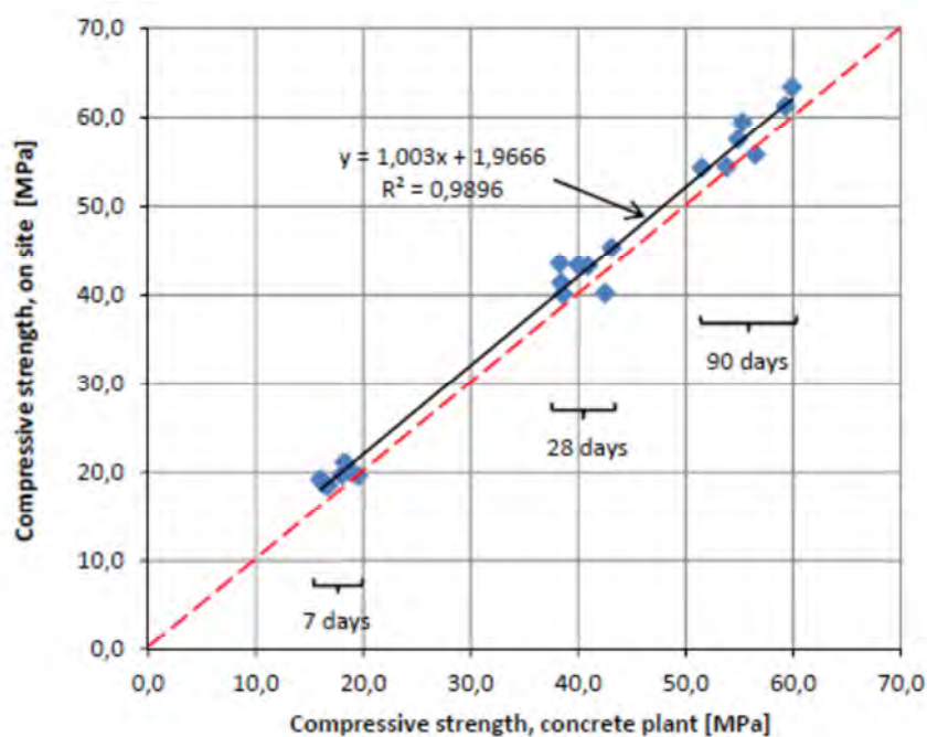
Figure 5-1. Comparison of compressive strength obtained at the concrete plant and at the Äspö Hard Rock Laboratory. From Mathern and Magnusson (2015).
