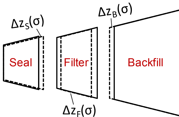
Figure 8.2. Illustration of the length change for the different components of the plug system during homogenization of the bentonite, from Börgesson et al. (2015a).
