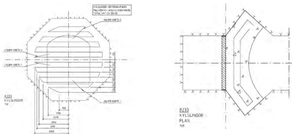
Figure 6-21. Cutout from construction drawing for placement of cooling pipes in the concrete dome. Left: front view, Right: horizontal cross-sectional view. (Text in Swedish)
