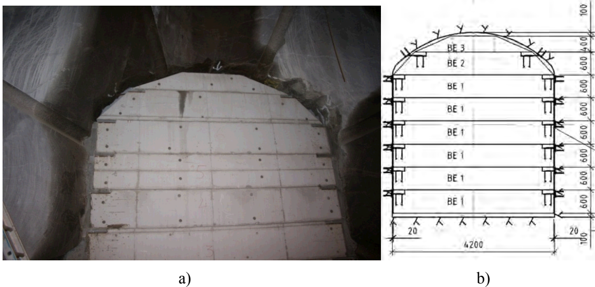
Figure 6-18. a) Installed concrete beams (the delimiter between bentonite seal and concrete dome). b) Sketch showing construction plan drawing of the concrete delimiter.
