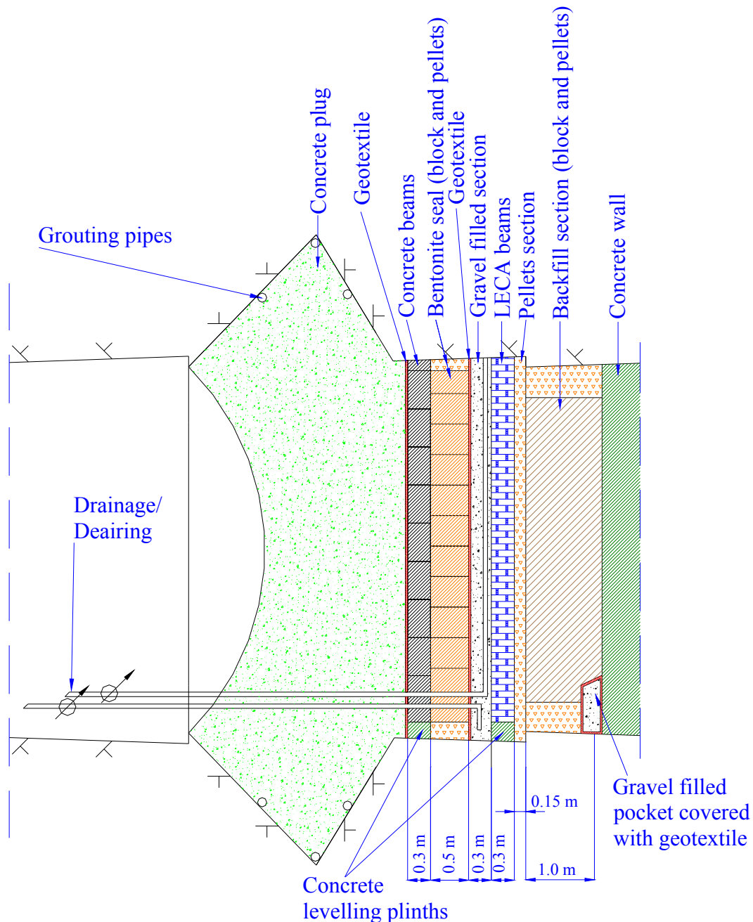
Figure 4-6. Layout of DOMPLU with its stiff draining material and the geological material that will drain the system to prevent a water pressure build-up on the concrete dome before it has hardened. The bentonite blocks will eventually swell and seal off water flow past the seal. The concrete beams will act as mechanical support.
