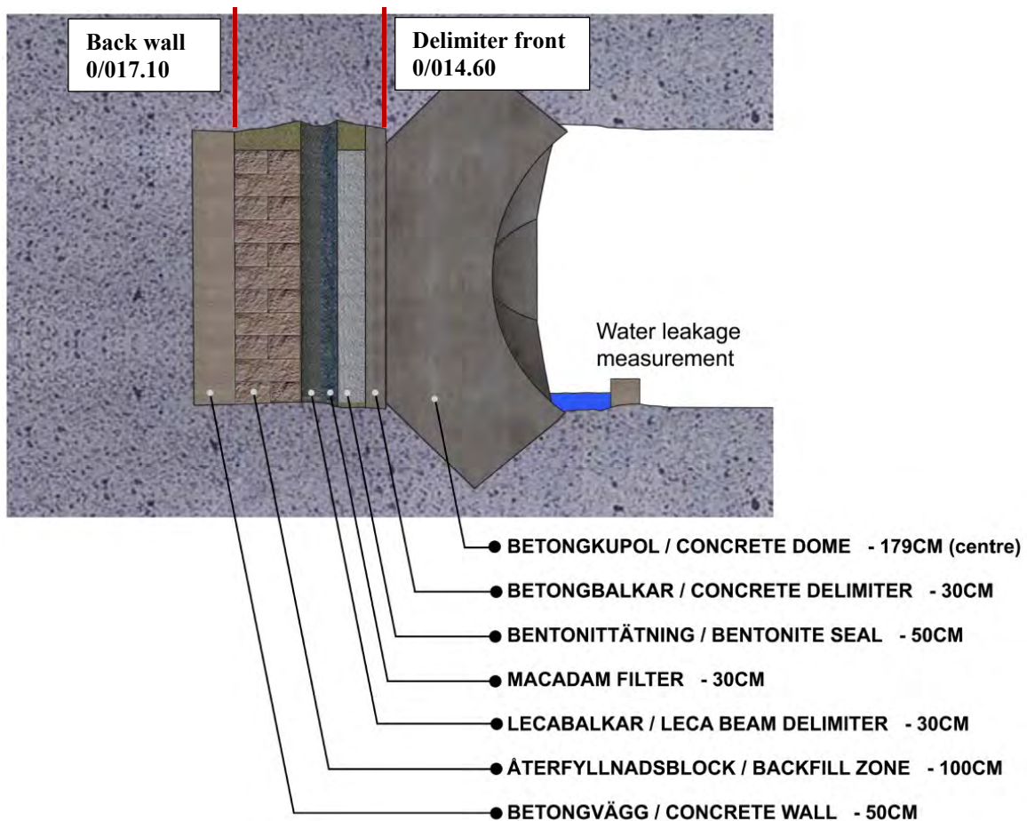
Figure 6-1. Sketch of the DOMPLU full-scale test in experiment tunnel TAS01, with fixed length-coordinates (Äspö 96) for the front delimiter and for the concrete back wall.
